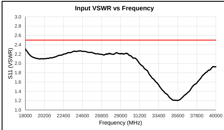
Typical Performance @ 23°C (Reference S/N 2332804)
