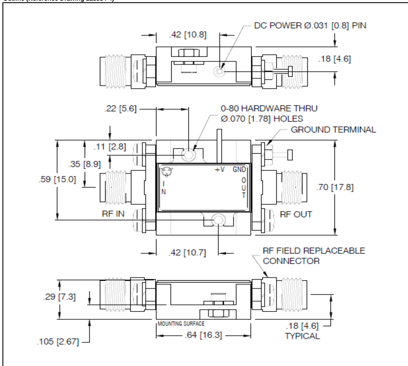
Outline (Reference Drawing 113384-4)
