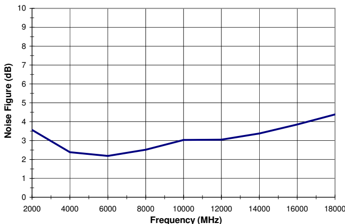
Noise Figure
