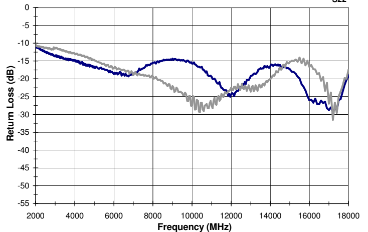
S11 & S22
