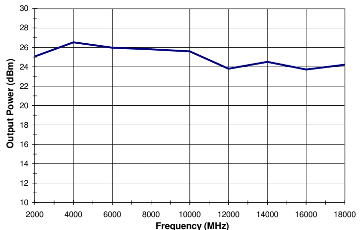
Output Power @ 1 dB Compression
